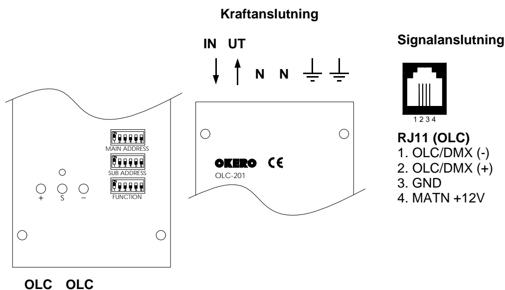
Figur 1. OLC201 inkoppling
